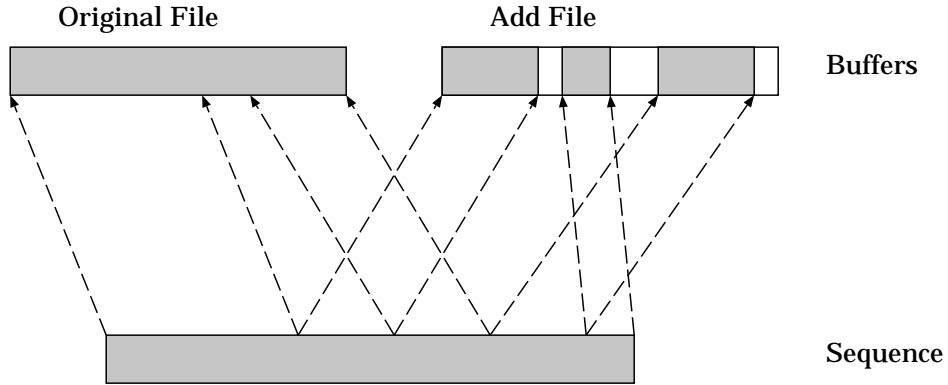
Figure 7: The piece table method
