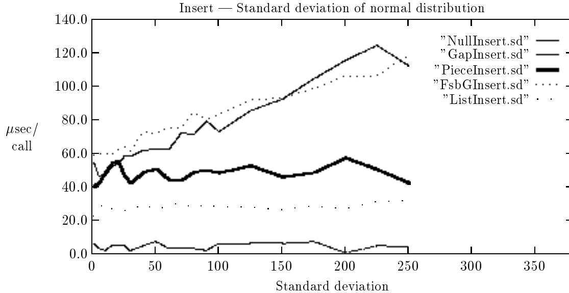
Figure 15: Insert times as the standard deviation varies
