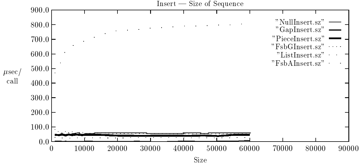
Figure 13: Insert times as the size of the sequence varies
