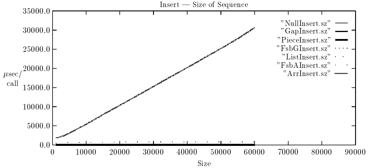
Figure 14: Insert times as the size of the sequence varies
